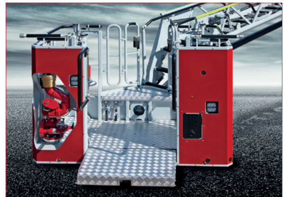
Newly developed rescue cage RC500-H
